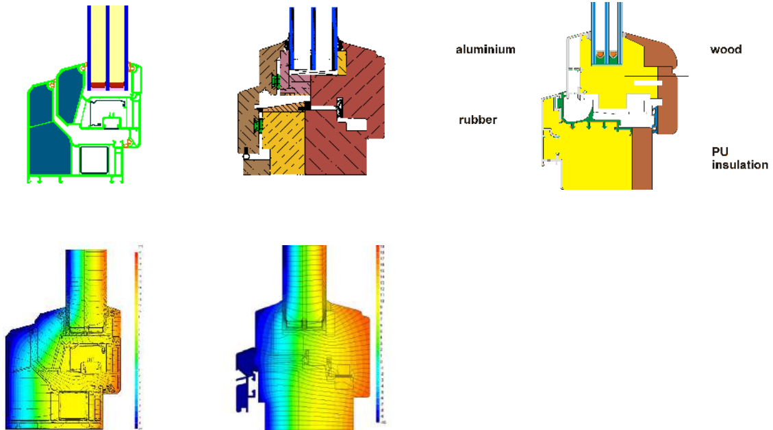
Figure 5: sample details of triple glazing in a window frame ( U=0,8 \text{ W}/(\text{m}^2\text{K}) ) Source: Passiv Haus Institut PHI, Passiefhuis-Platform vzw
